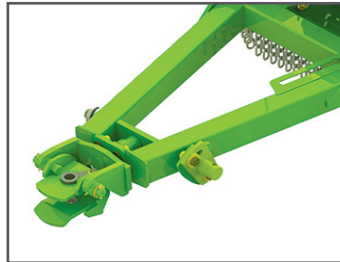
Pro Level Hitch Fits Cat 2 and Cat 3 is one of five optional Hitches
