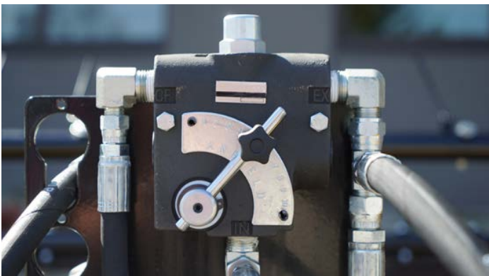
HYDRAULIC DRIVE
