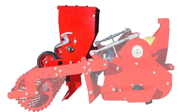
Pro Grass Seeder: for grass wheat, corn, peas, hemp, sorghum, alfalfa and onions. Option for all Rotex and Yellowstone models
